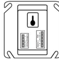
CM-6 rear view with Modular Connectors
